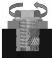
Clamp load torque
